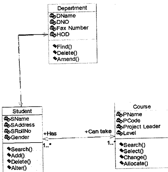
Class diagram for student info system
