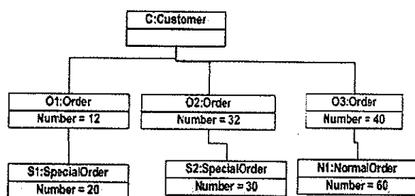
Object diagram of an order management system
