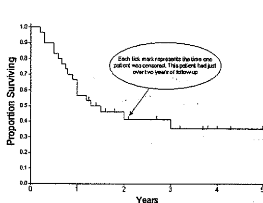
Figure-6 (a): Samples of Kaplan-Meier survival curves.
