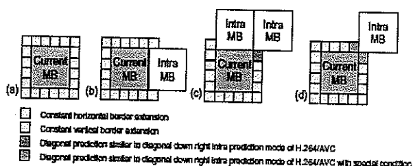
Figure 4 : Padding of Intra Macroblocks Before Upsampling
