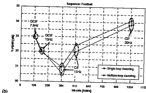
Figure 5 : Coding results for the sequence Football
