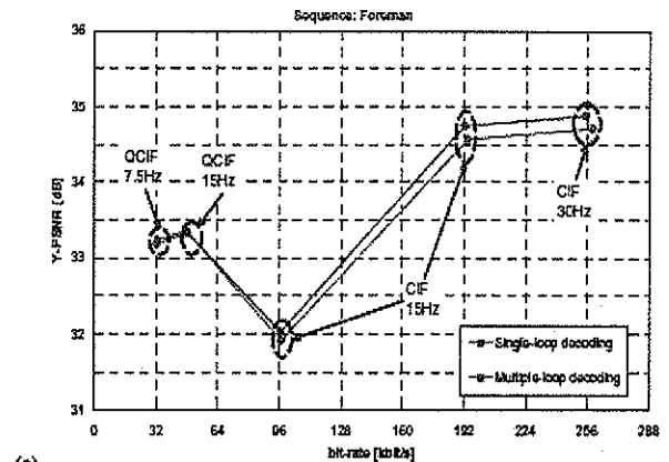
Figure 5 : Coding Results for the Sequence Foreman
