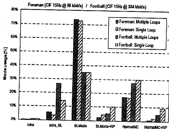
Figure 6 : Mode usage for the first CIF 15 Hz layer
