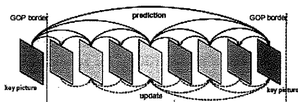
Figure 2 : Hierarchical Prediction Structure
