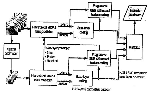
Figure 1 : Typical coder structure for the scalable extension of H.264/AVC
